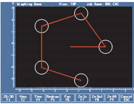
Bolt Hole Drilling and Threading Cycles
