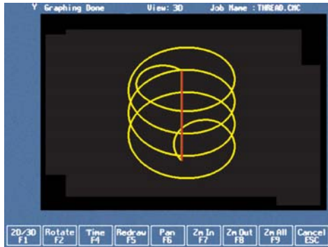
Thread Milling
