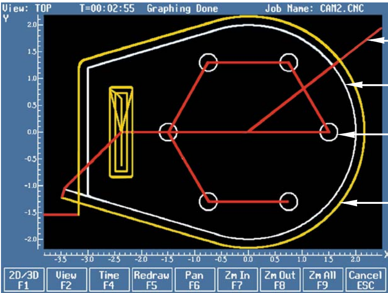
Thread Milling
