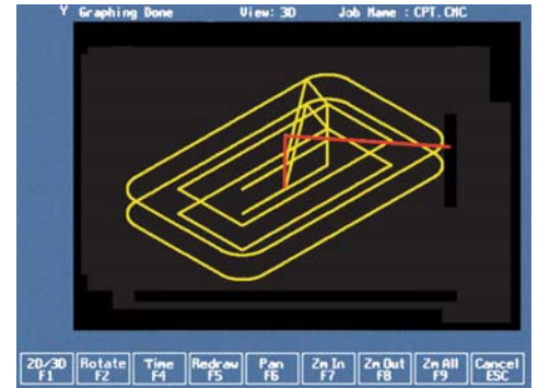
Rectangular/Circular Pocket Milling
